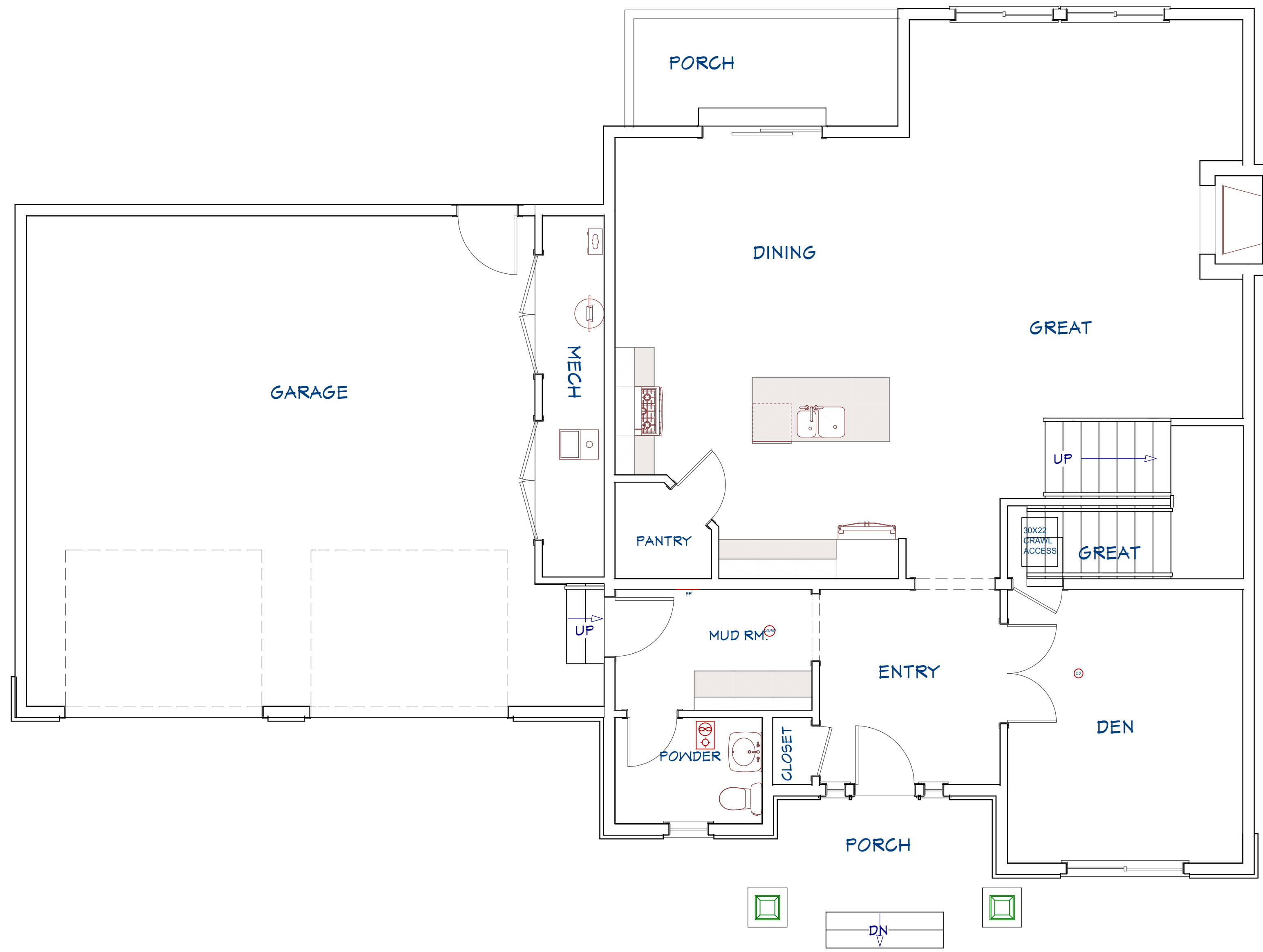
Main Floor M/E/P Plan 1/4 in = 1 ft
