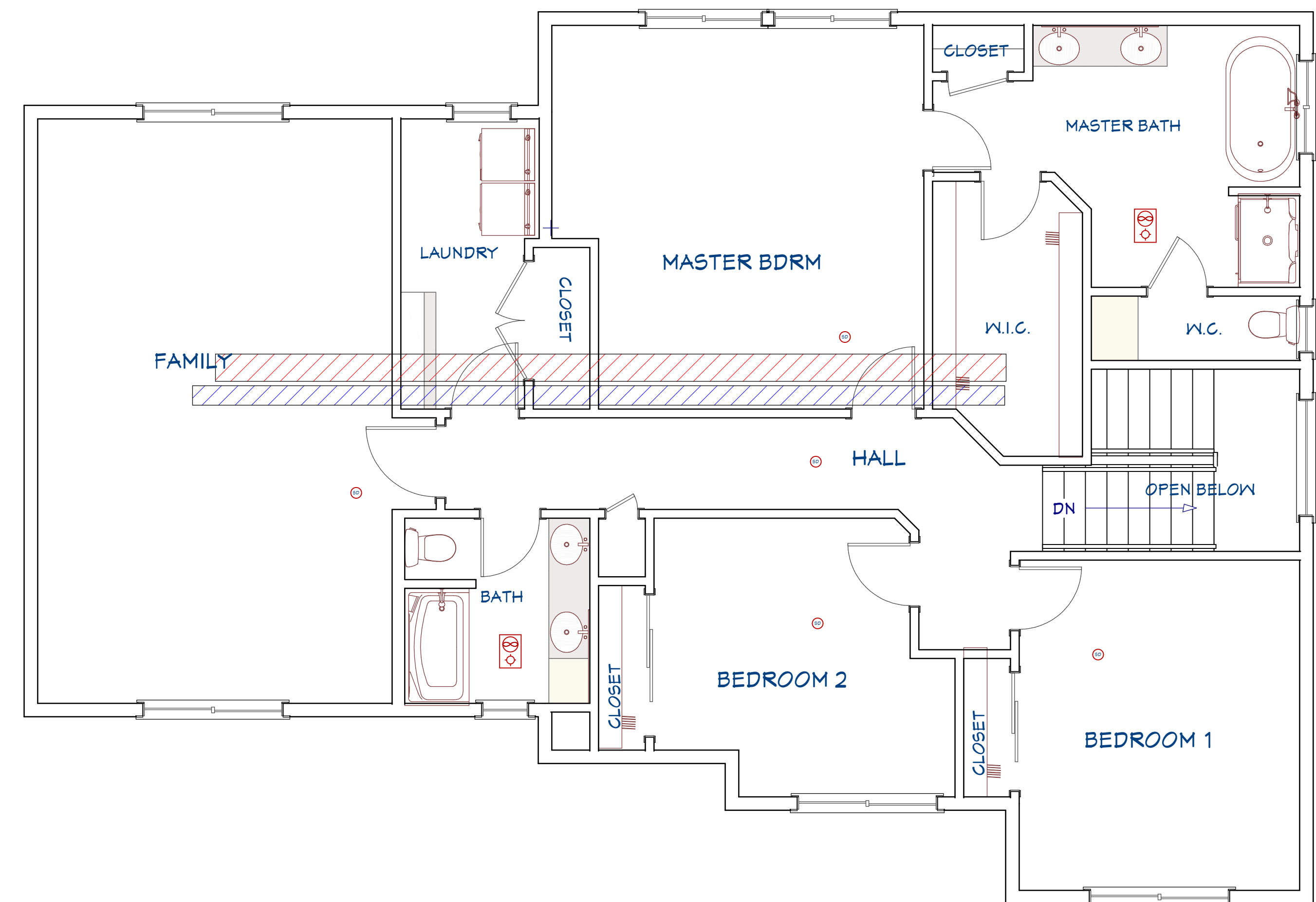
2nd Floor M/E/P Plan 1/4 in = 1 ft
