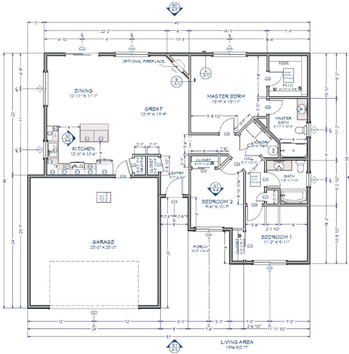
Main Floor Plan 1/4 in = 1 ft
